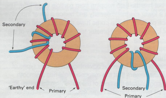
Two possibilities of winding an 8:2 transformer for RF.
