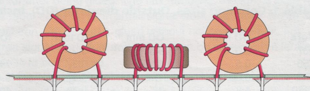
Optimum positioning for minimum coupling in critical applications.
